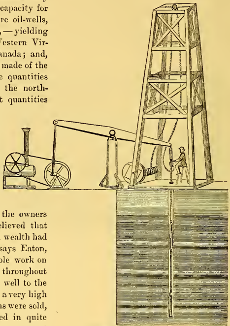
PROCESS OF BORING FOR PETROLEUM.
